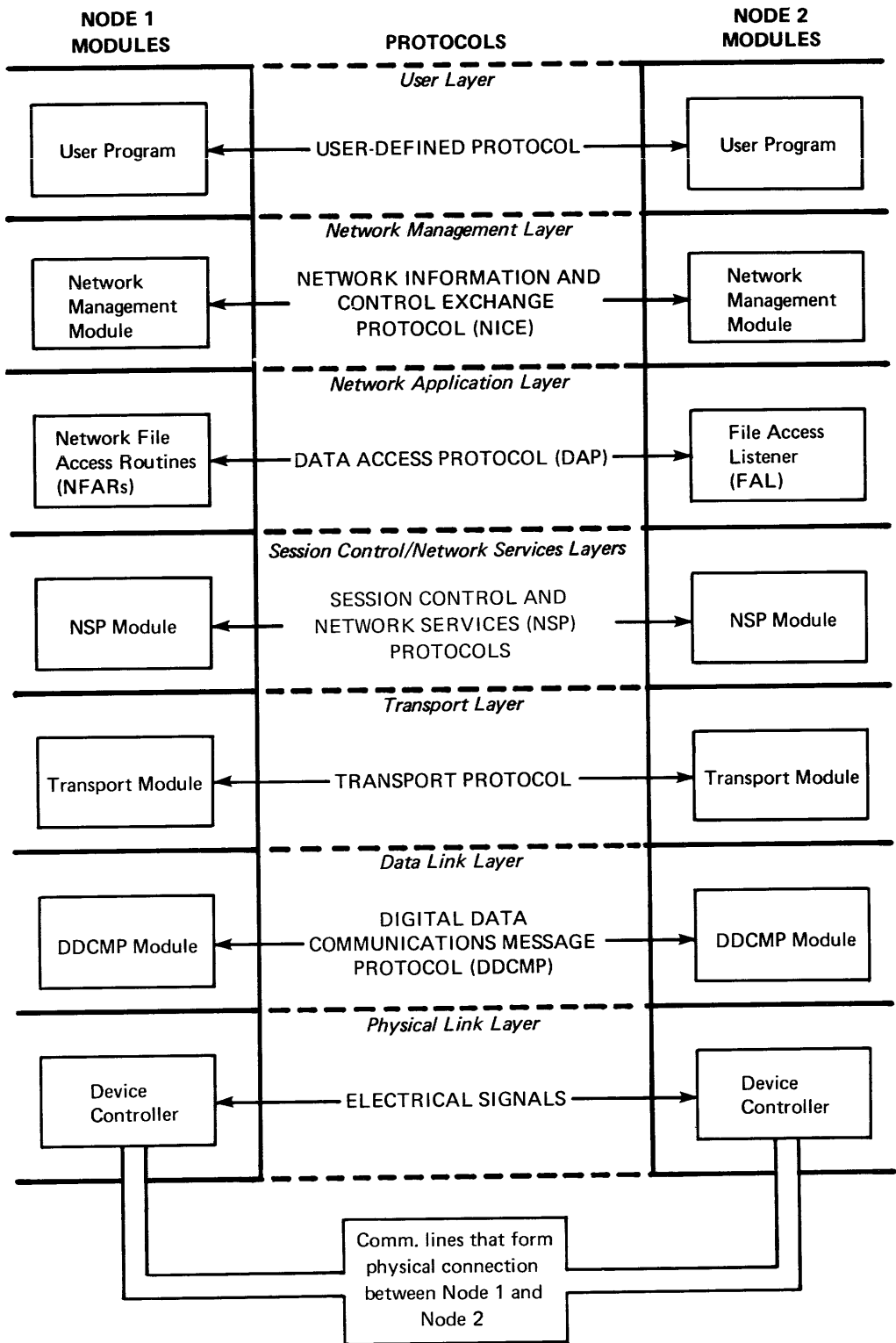
Figure 2-3: Protocol Communication between Equivalent Modules
