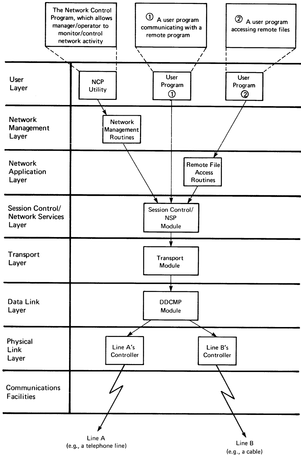
Figure 2-2: Vertical Interaction of DECnet Software Modules
