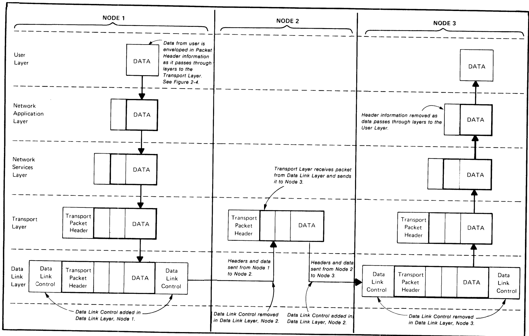
Figure 2-5: Data Flow from Node 1 to Node 3 in a Three-Node Network
