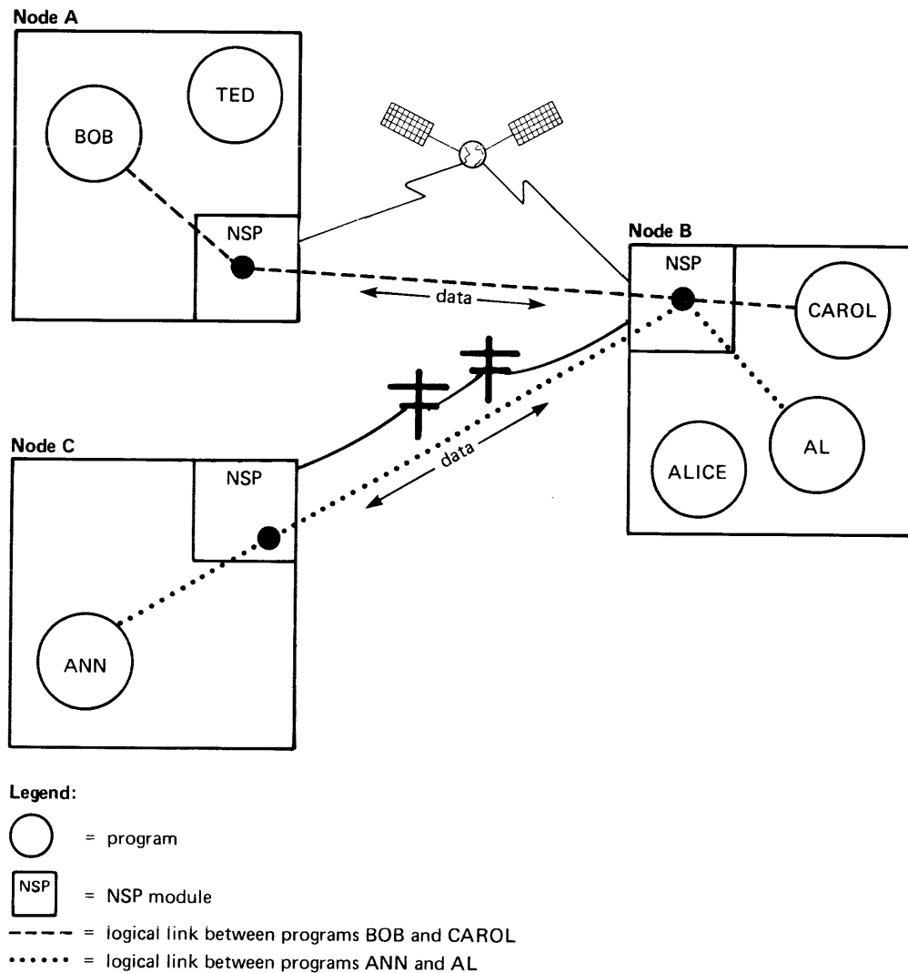
Figure 4-2: NSP Modules and Logical Links
