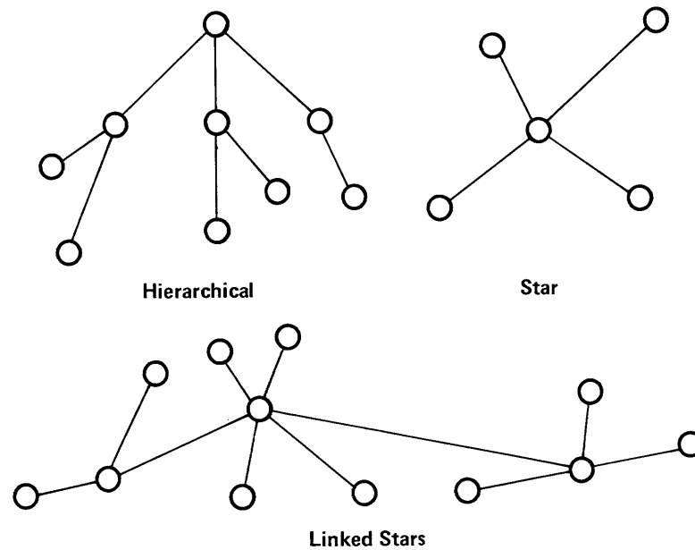
Figure 3-3: Phase II DECnet Configurations
