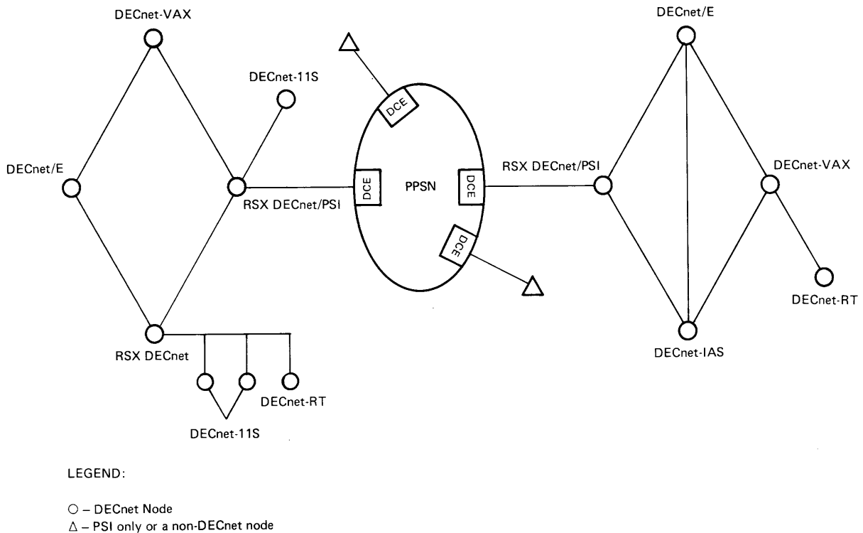
Figure 3-11: RSX DECnet/PSI Nodes within a Phase III Network
