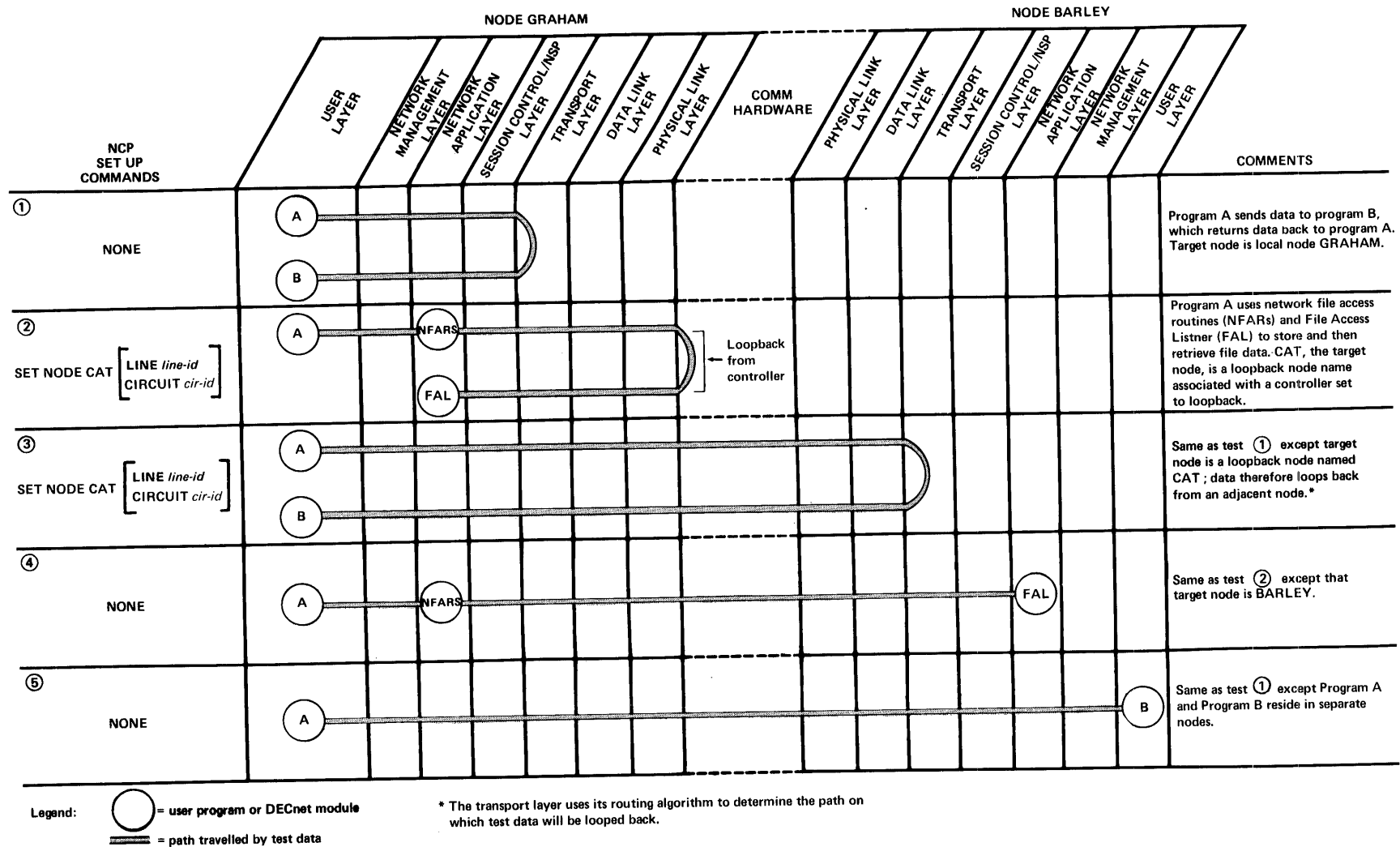
Figure 10-3: Program-initiated Loopback Tests
