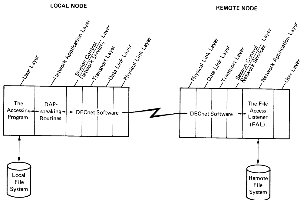
Figure 6-1: Remote File Access
