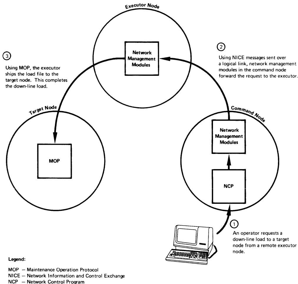
Figure 9-1: A Down-line Load Initiated by a Command Node
