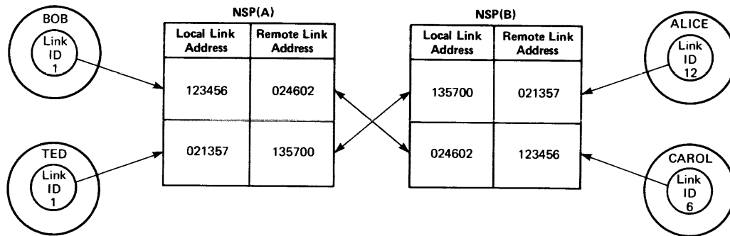
Figure 4-3: Interrelationship of Link Identifiers and Addresses
