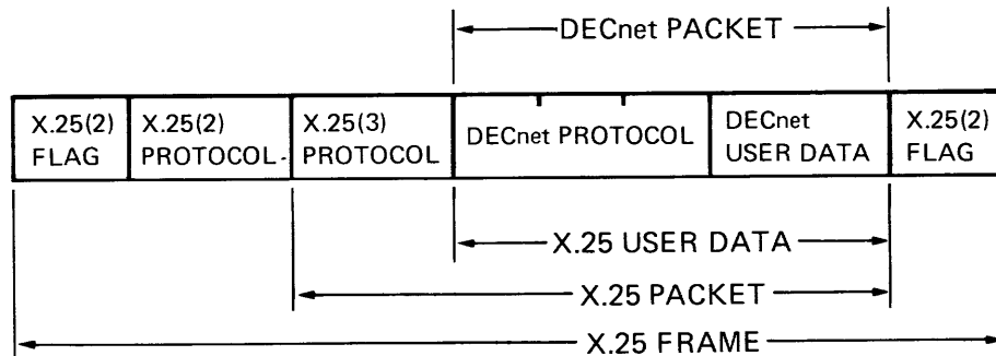
Figure 3-9: A DECnet Packet Nested in X.25 Protocol
