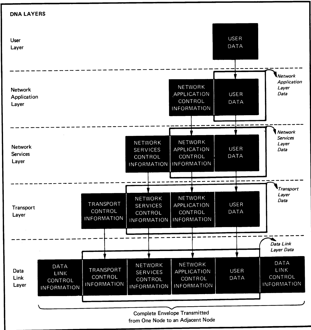
Figure 2-4: Enveloping User Data in Protocol
