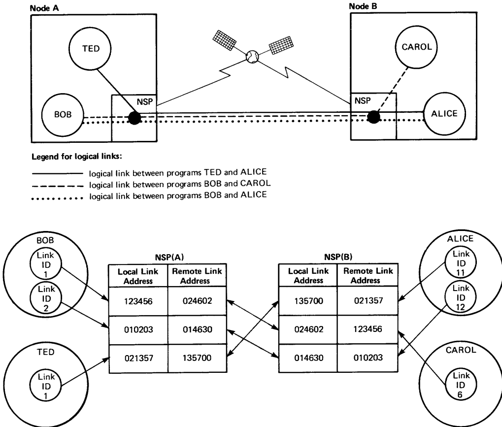
Figure 4-4: Programs Supporting Multiple Logical Links
